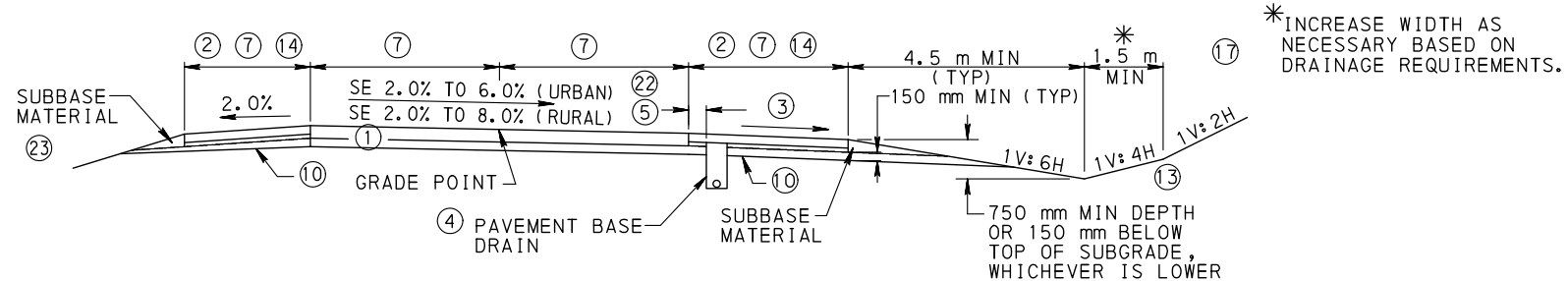
TYPICAL SUPERELEVATED SECTION
