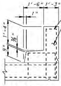
SECTION A-A EXISTING BARRIER
