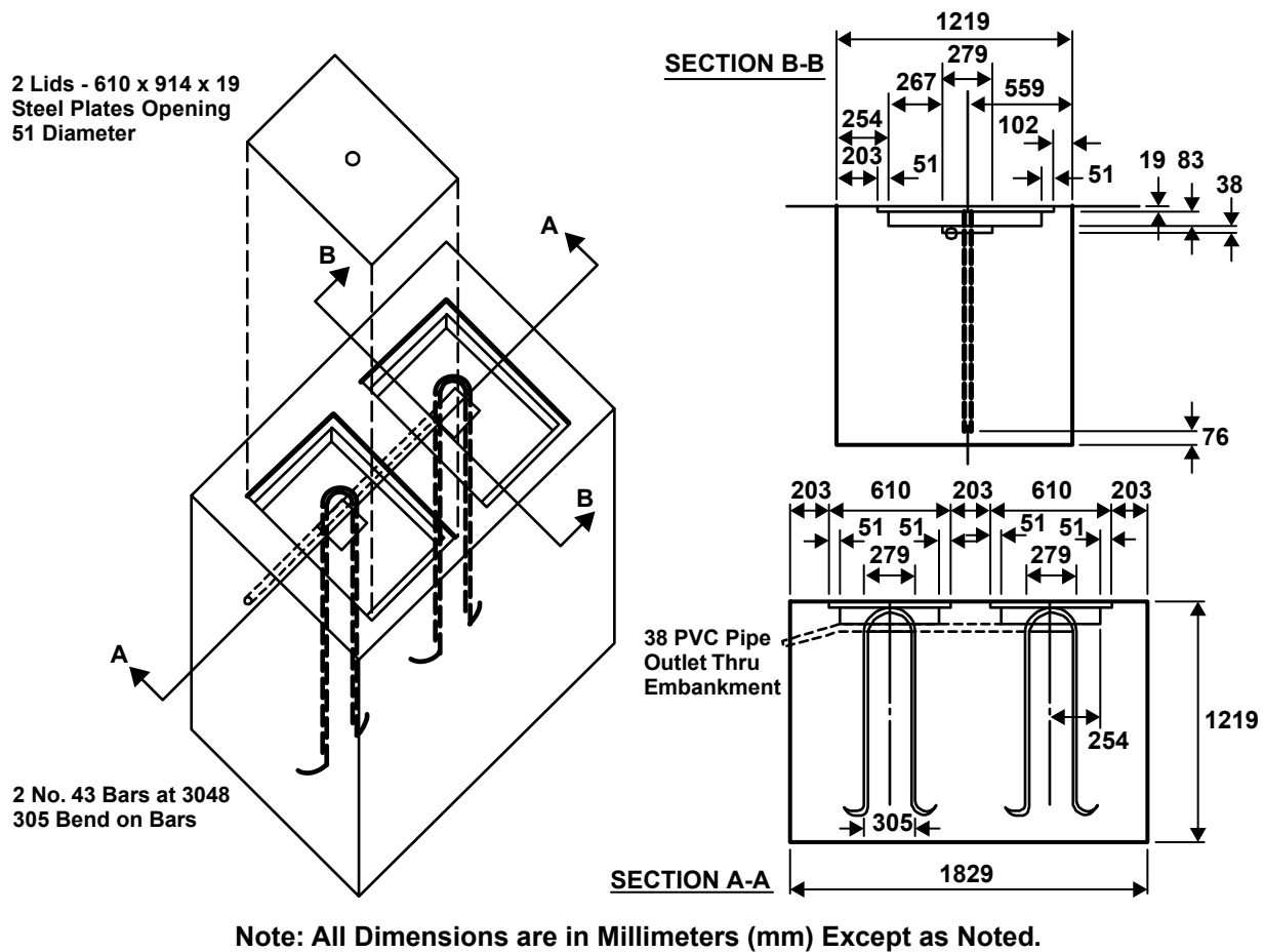
FIGURE 17.12 (METRIC) Design of a Concrete Anchor Block Dead Man
