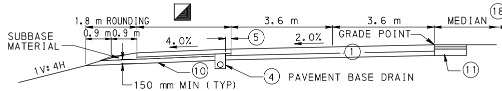
TYPICAL FILL SECTION--4.5 m AND UNDER
