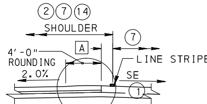
TYPICAL SUPERELEVATION SECTION SE > 6.0%
