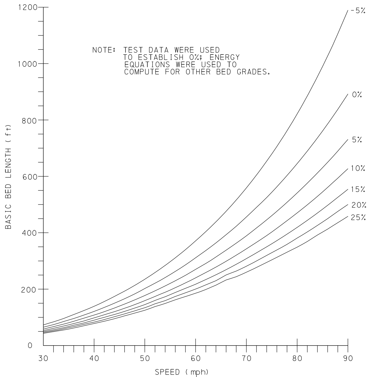
FIGURE 17.1 (ENGLISH) EFFECT OF GRADE ON RIVER GRAVEL BED
