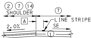
TYPICAL SUPERELEVATION SECTION SE 2.0% TO 6.0%
